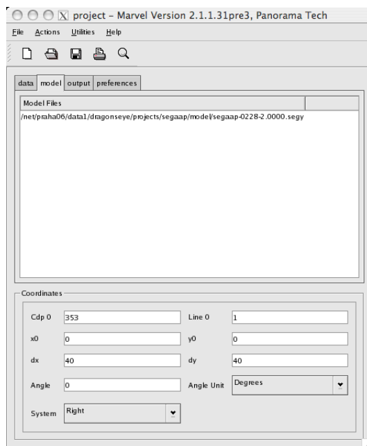
Figure 3. Project Window with Model Pane
