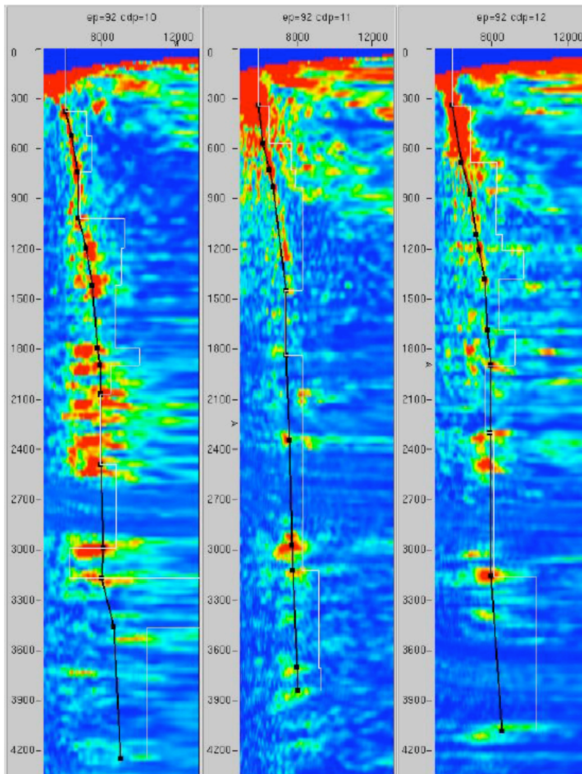
Figure 42. Picking an initial velocity model from topography
