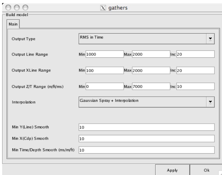
Figure 28. Build Model Window
